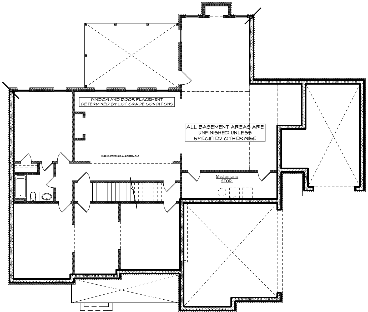
FOUNDATION/TERRACE LEVEL FLOOR PLAN
